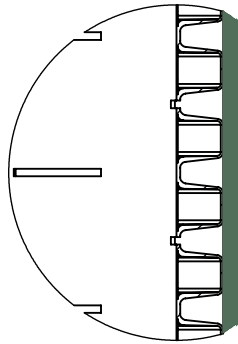
DETAIL G SCALE 2 : 3
