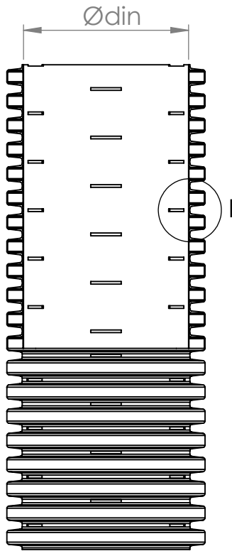
SECTION H-H
