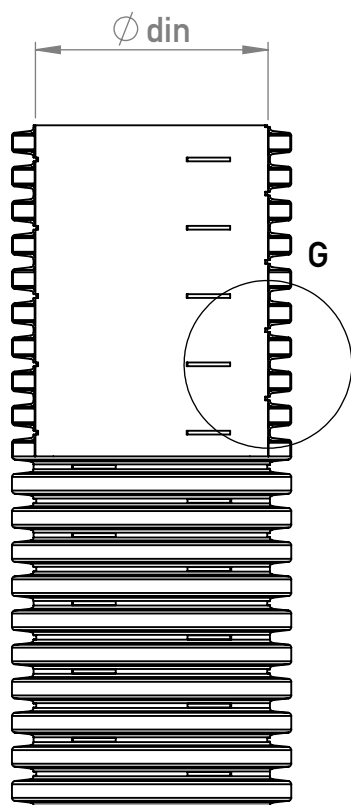
SECTION F-F
