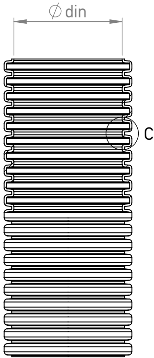
SECTION B-B
